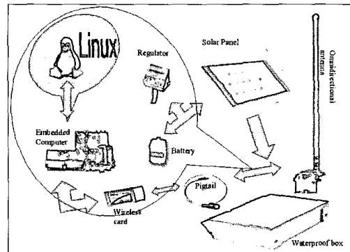
Figure 2: Design of the wireless solar-powered router
