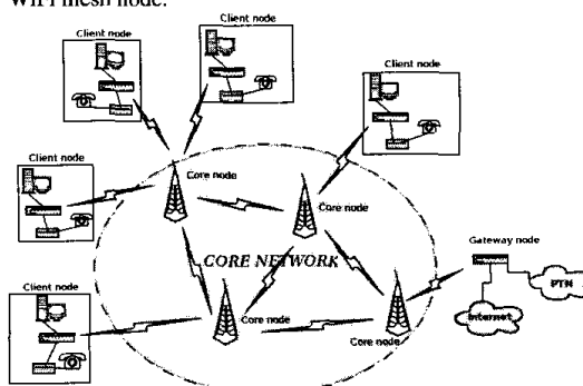
Figure 1: Mesh Network Architecture
