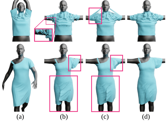
Figure 3: Unposing of a T-shirt and a dress in challenging poses: (a) input mesh; (b) unposing with constant weights [41, 53], notice the collisions; (c) unposing with variable weights assigned with nearest vertex, it avoids collisions but introduces skinning artifacts and is not temporally stable, better seen in video; (d) unposing with our optimization.
