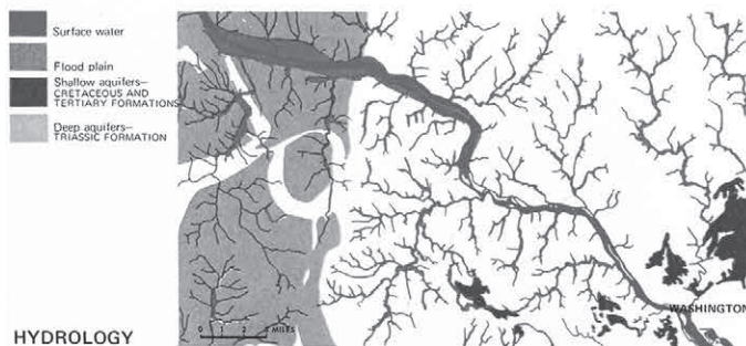
HYDROLOGY
