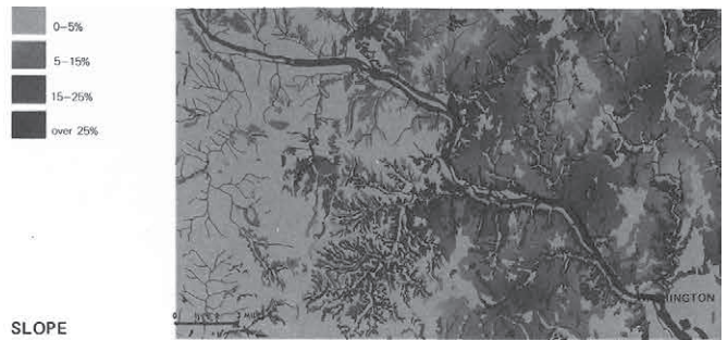
SLOPE
