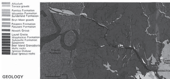
GEOLOGY
