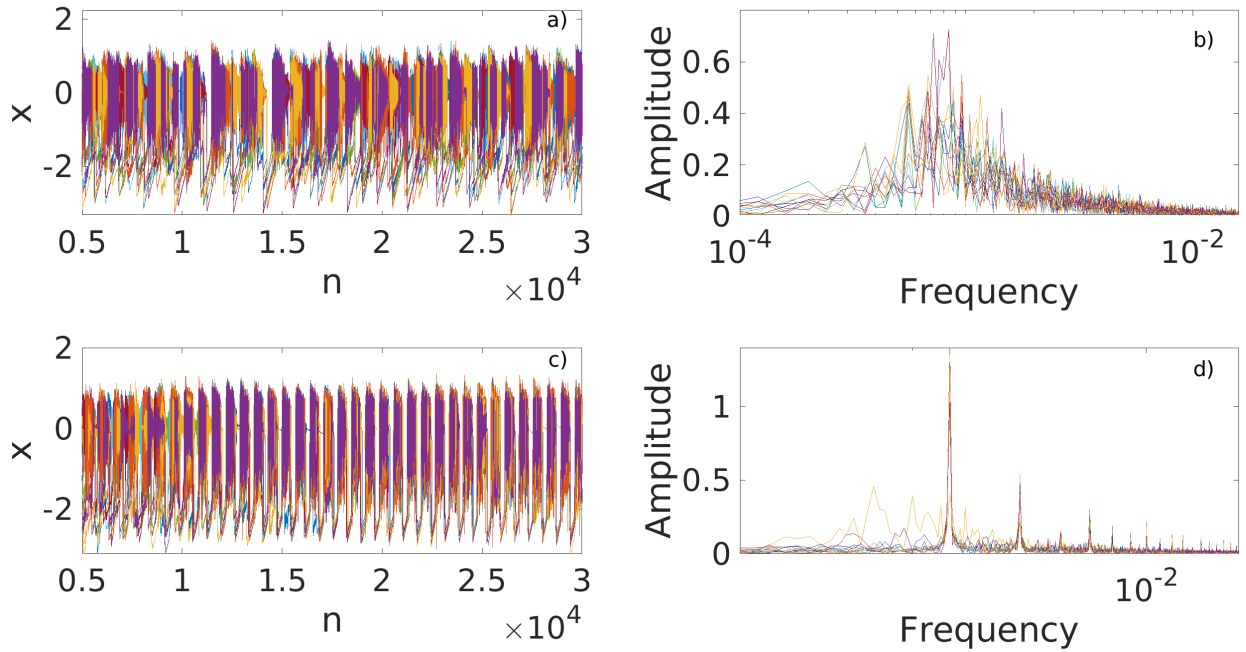
Figure 8. Time series (left panels) and Fourier transform (right panels), for the small-world network with a low noise intensity in \alpha . Panels (a-b) represent the dynamics without using the delay, while in panels (c-d) we use the delay. The parameter values are: N = 50 , p = 0.2 , k = 2 , \alpha_0 = 3.75 and D = 0.1 . Each color represents one fundamental frequency. In (a), there is no synchronization, and in (b) there is a great frequency dispersion. However the network can be synchronized by using the delay, as shown in (c) and (d).
