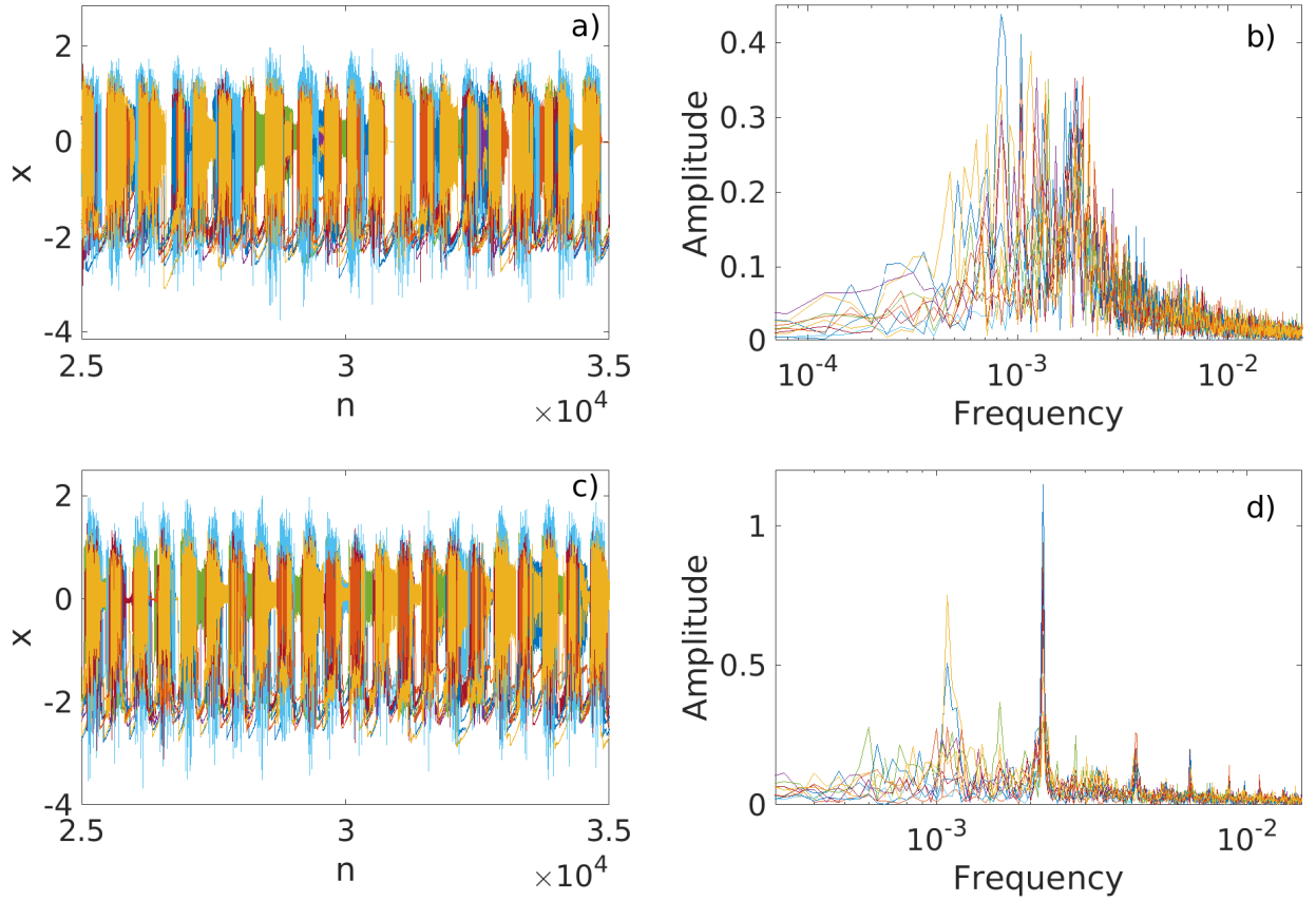
Figure 10. Time series (left panels) and Fourier transform (right panels) for neurons in a small-world network with a high noise intensity in \alpha . The upper panels were computed without using delay and the lower panels using the delay. The parameter values are: n = 50 , p = 0.2 , k = 2 , \alpha_0 = 3.75 , and D = 0.75 . Each color represents one fundamental frequency. In this case the delay cannot synchronize all neurons.
