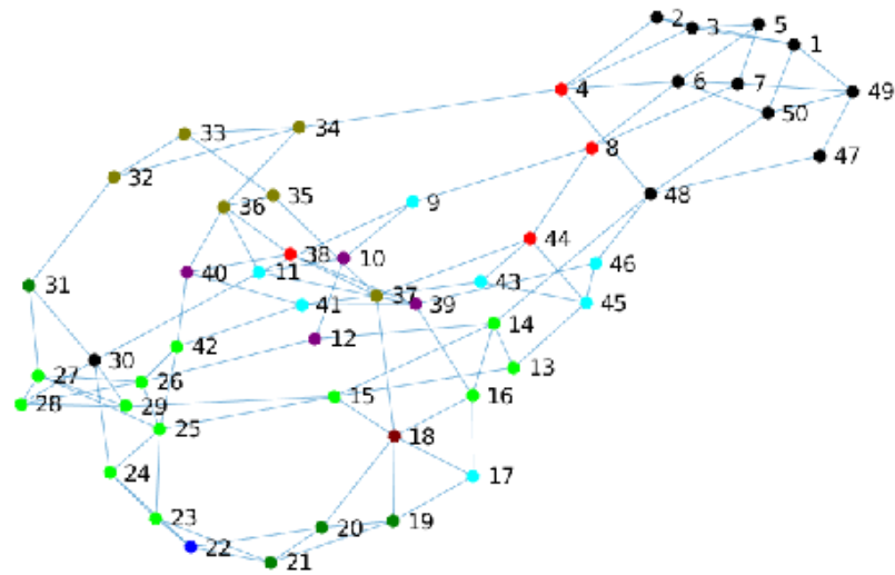
Figure 4. Graph used in our simulation with a small-world network. Colors represent the different fundamental frequencies of each neuron for \alpha = 3.75 , illustrating that the neurons with similar fundamental frequencies are clustered.
