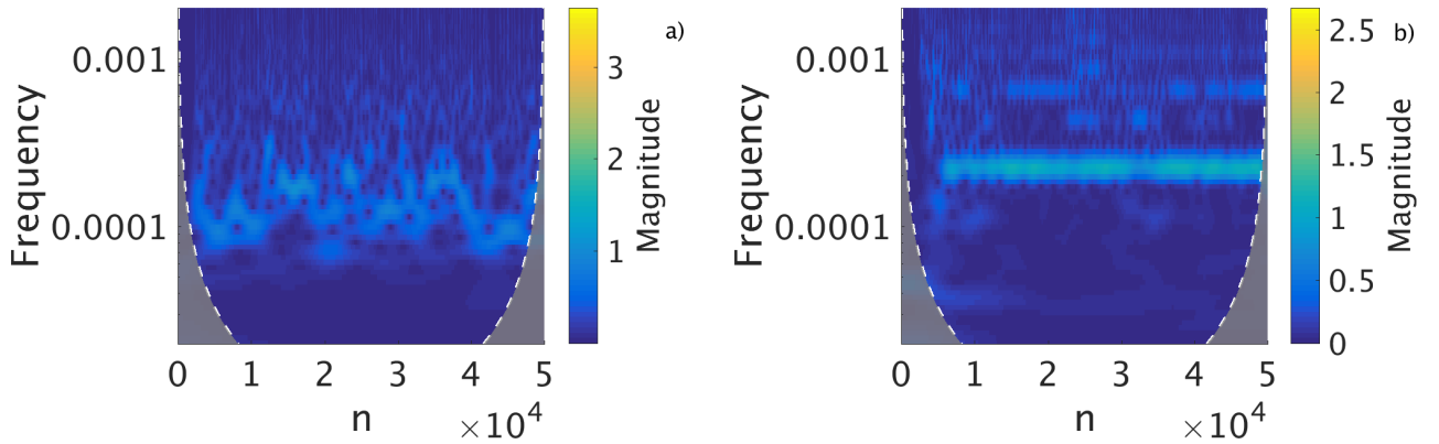
Figure 12. Wavelet transform for a random neuron extracted from our simulation with a high noise intensity in \alpha . As usual, the left panel is without delay and the right panel with it. As in the previous cases, the grey region represents the points that are not reliable. In (a) we do not see any steady frequency, while in (b) we can see a steady fundamental frequency, though this does not happens for its harmonics.
