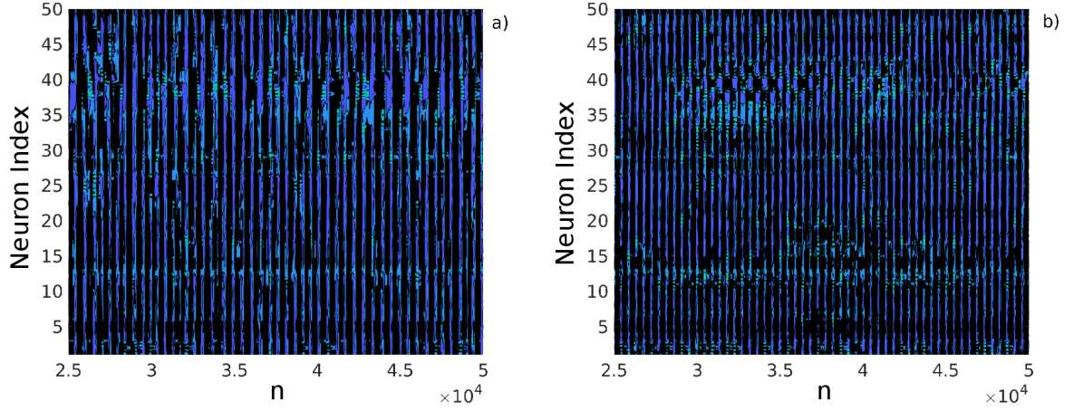
Figure 11. Space-time plots of our small-world network obtained from our simulation with a high noise intensity in \alpha . The left panel shows the case without delay and right panel the case with delay. Some sort of synchronization can be observed in (a), while in (b) the synchronization seems to have been improved.
