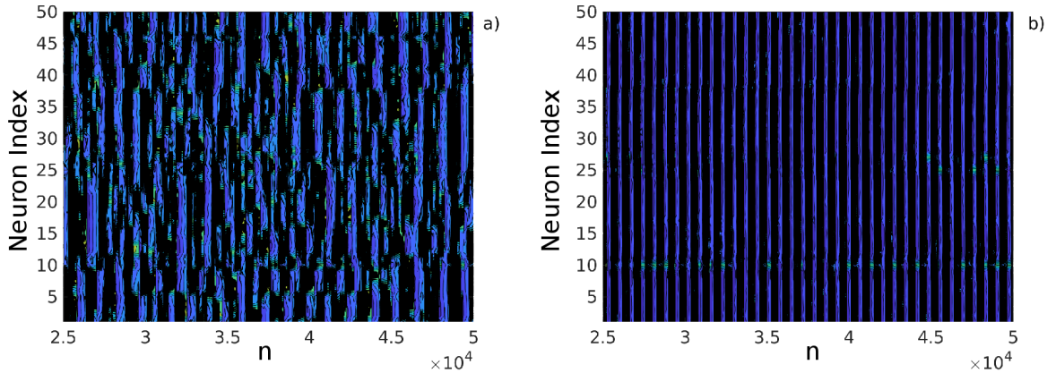
Figure 9. Space-time plots of our small-world network obtained from our simulation with a low noise intensity in \alpha . Left panel without delay and right panel with delay. In (a) there is no synchronization, but in (b) the network gets synchronized as if there were no noise.
