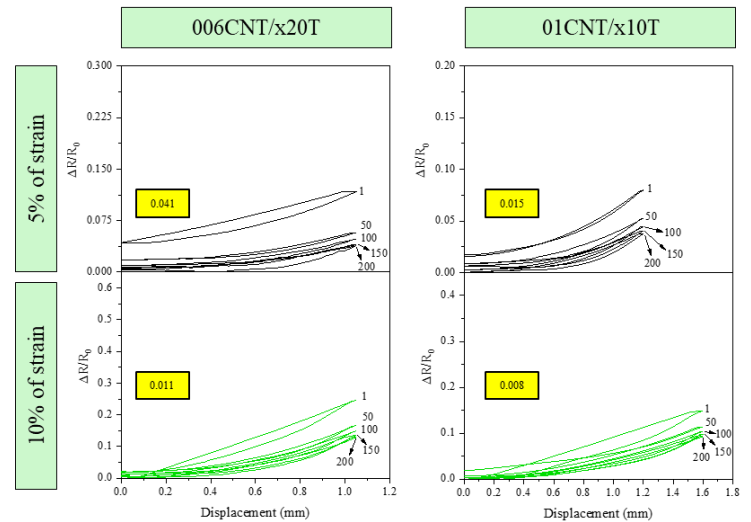
Fig. 13. Hysteresis loop for the two conditions tested under cyclic tests. Five cycles are presented for each condition.
