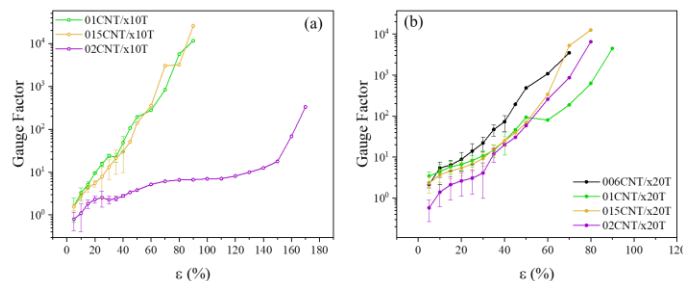
Fig. 9. GF values as a function of applied strain for (a) x10T and (b) x20T conditions.
