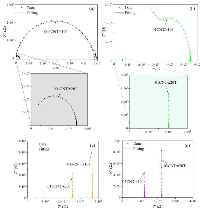
Fig. 5. Nyquist plots of (a) 0.06, (b) 0.1, (c) 0.15, and (d) 0.2 wt. % CNT samples where the solid symbols denote the x20T and the hollow ones the x10T samples.
