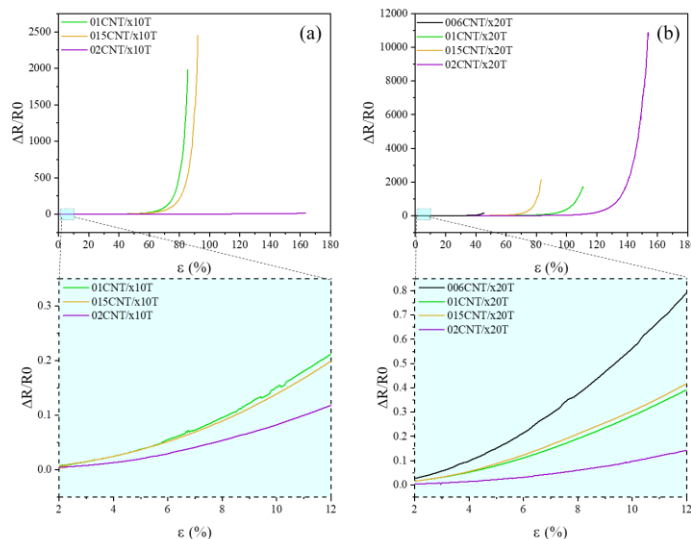
Fig.8. Electromechanical quasi-static tensile stress tests, where the electrical response with strain is observed for each sample for (a) x10T and (b) x20T conditions.
