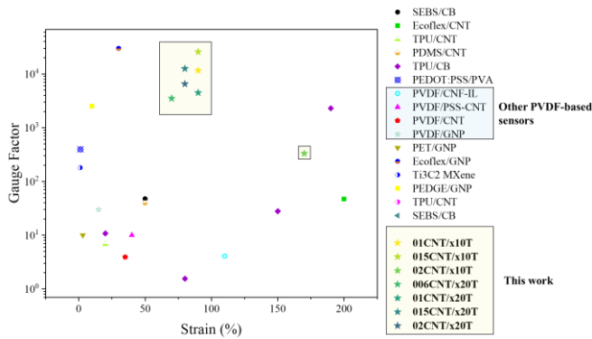
Fig. 10. Comparison of the relationships between gauge factors and strain values referenced in the literature and those obtained in this work.
