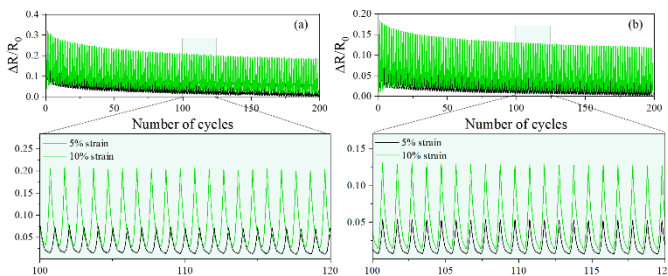
Fig.11. Electrical response during 200 cycles for (a) 0,06CNT/x20T and (b) 0,1CNT/x10T conditions.
