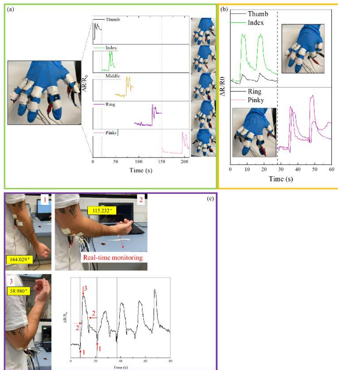
Fig.13. Electrical response of each sensor during the proof-of-concept testing for (a) independent movement of each finger, (b) movement of two fingers at a time, and (c) elbow movements
