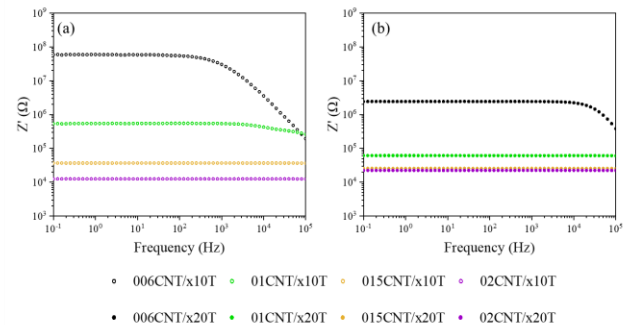
Fig. 4. Z' plots as a function of AC frequency for (a) x10T and (b) x20T samples.
